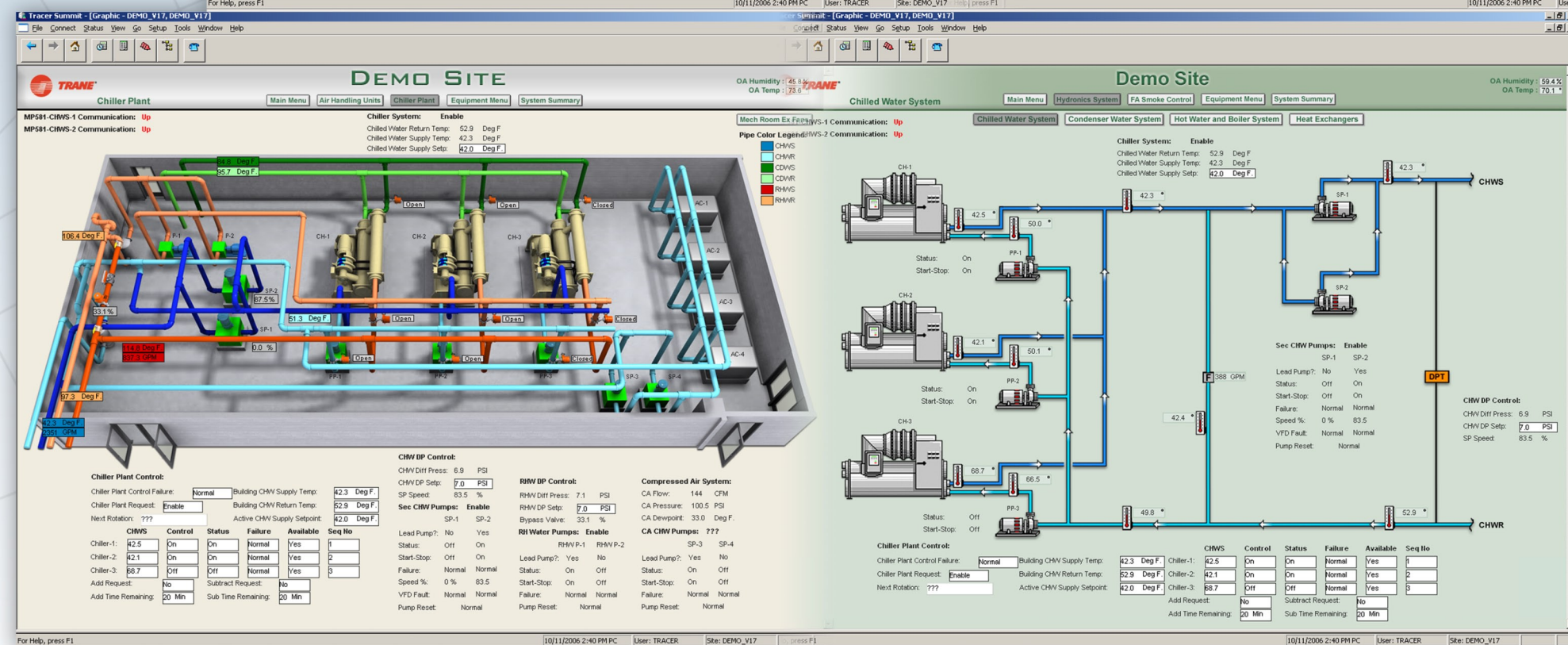
3D -HVAC Mechanical Room (Chiller Plant)-
